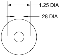
7 1/4" WASHER (1/16" THICK)
