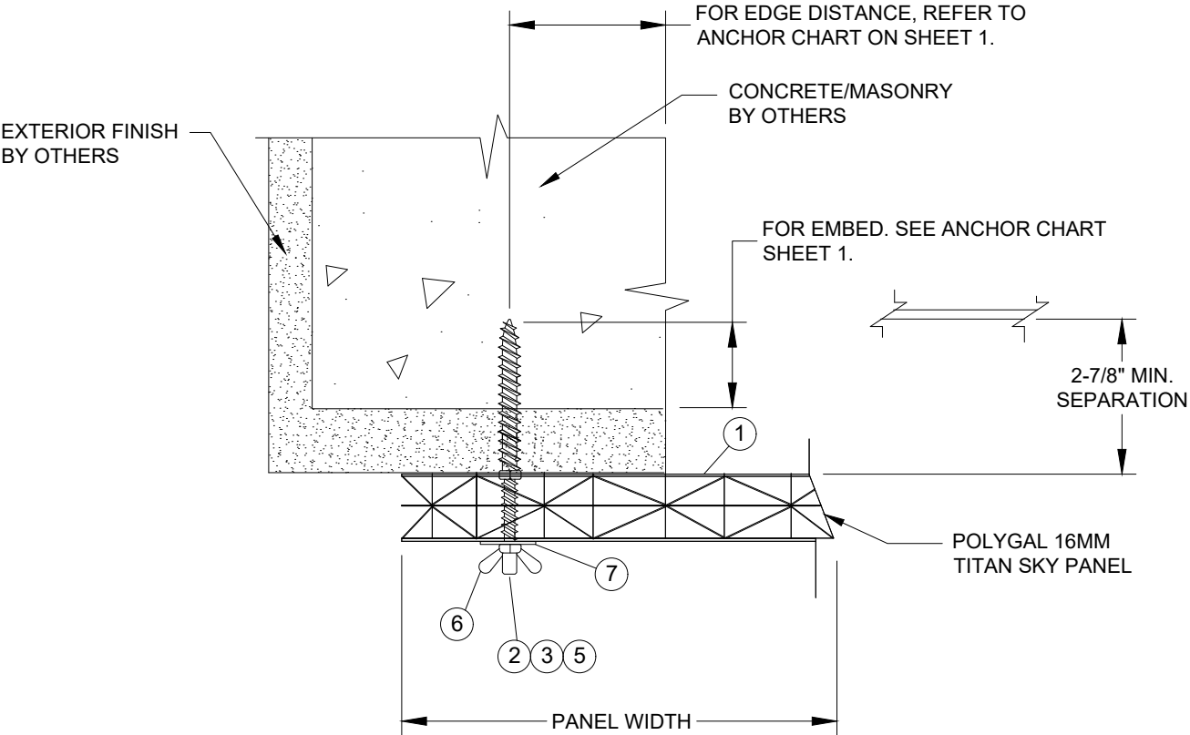
B 4 HORIZONTAL SECTION MASONRY/CONCRETE SUBSTRATE WALL MOUNT INSTALLATION
