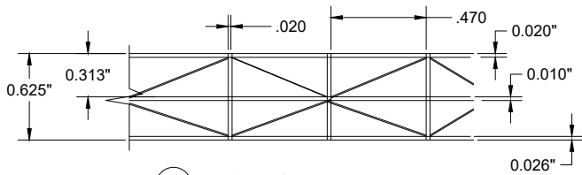
1 POLYGAL 16MM PANEL CROSS SECTION POLYCARBONATE
